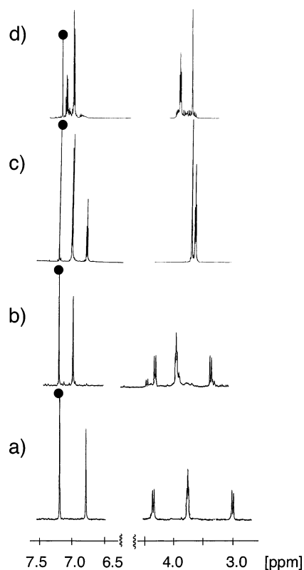
Figure 5. Portions of the ^1\text{H} NMR spectra (500 MHz, \text{CDCl}_3 , 295 \pm 1 K) of: (a) calix[4]arene 1 . (b) nitrosonium complex 7 ; the identical spectrum was obtained upon addition of \text{NO}^+\text{SbF}_6^- to 1 . (c) calix[4]arene 2 . (d) nitrosonium complex 8 ; the identical spectrum was obtained upon addition of \text{NO}^+\text{SbF}_6^- to 2 . The residual \text{CHCl}_3 signals are marked “●”.
