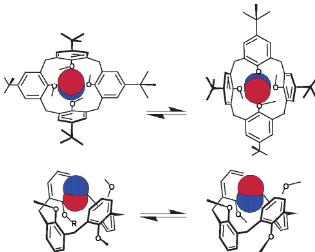
Figure 6. Proposed host–guest dynamics in calix[4]arene–NO + complexes.
